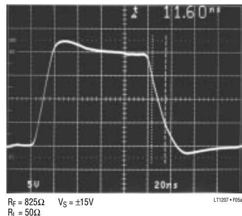
Figure 5a. Large-Signal Response, A_V = 1
