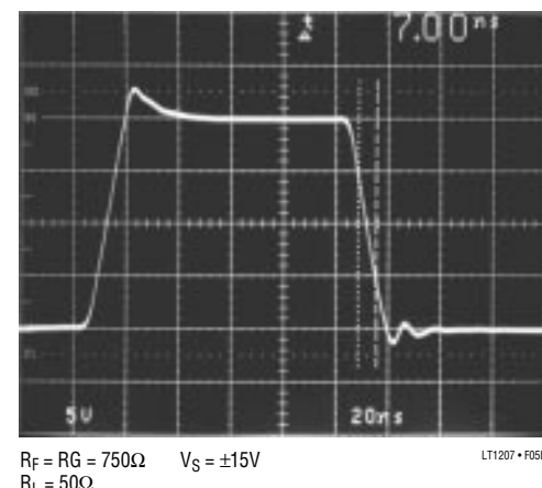
Figure 5b. Large-Signal Response, A_V = -1
