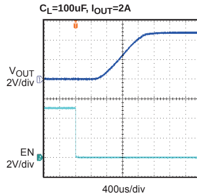
Turn On Delay and Rise Time with 100uF Load
