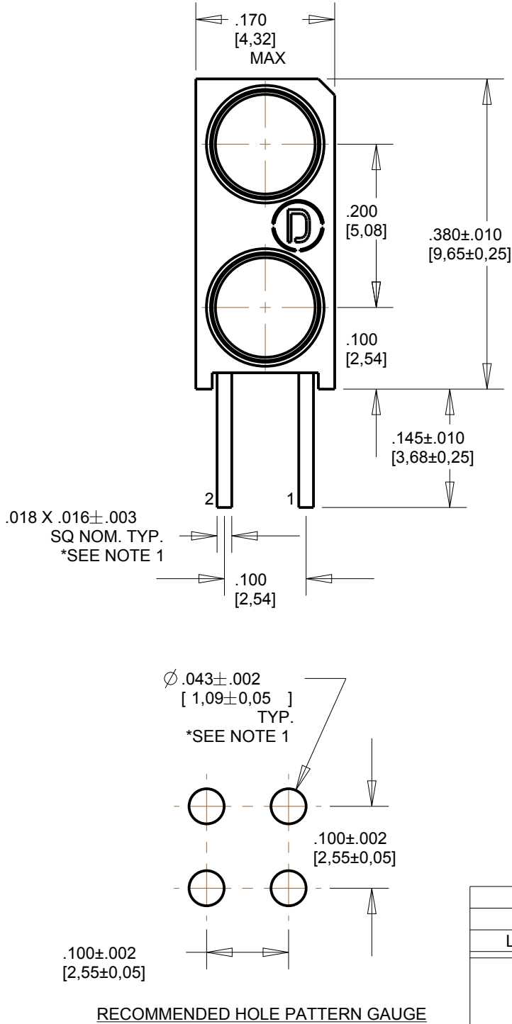
RECOMMENDED HOLE PATTERN GAUGE
