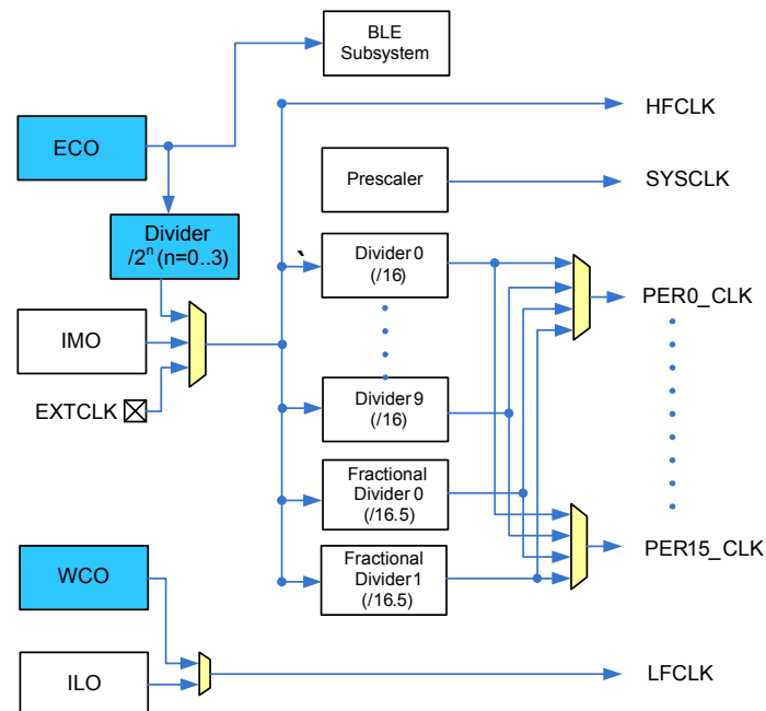
Figure 2. Clock Control
