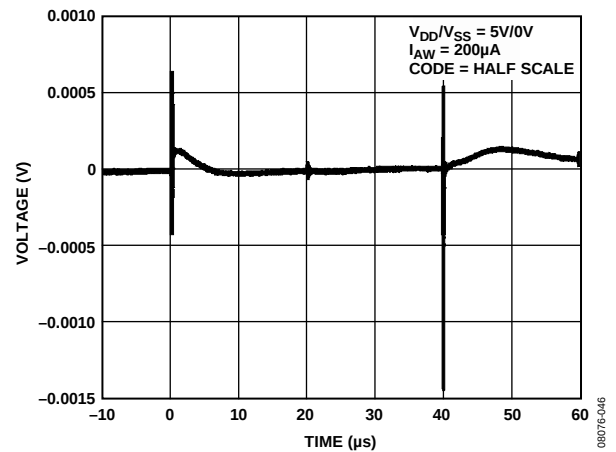
Figure 34. Digital Feedthrough
