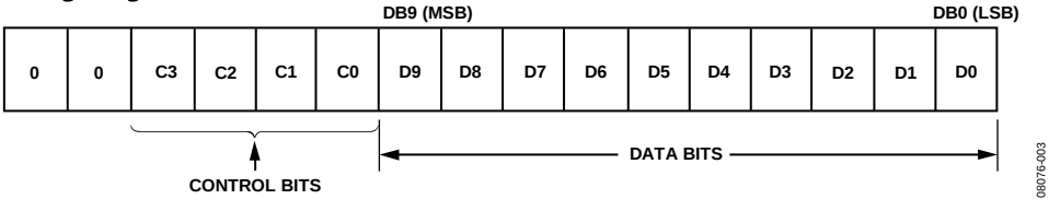
Figure 2. Shift Register Content
