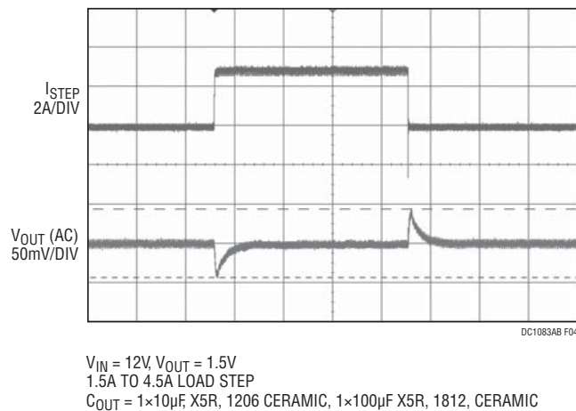
Figure 4. Measured Load Transient Response (3A Step)
