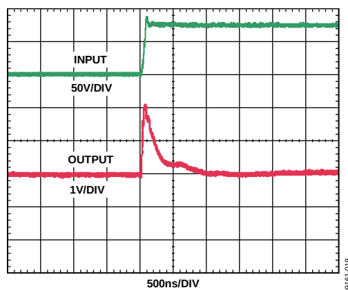
Figure 19. Common-Mode Step Response, Rising
