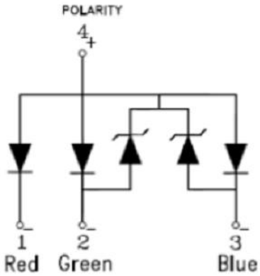
LED SCHEMATIC
