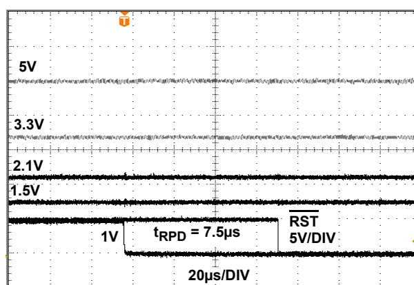
FIGURE 6. ISL88031 t_{RPD}
