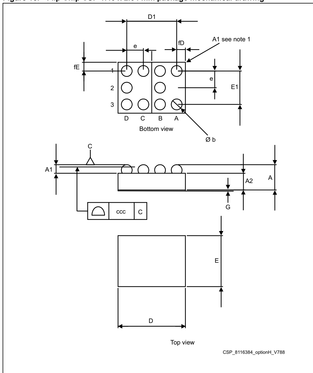
Figure 15. Flip Chip CSP 1.40 x 2.04 mm package mechanical drawing
