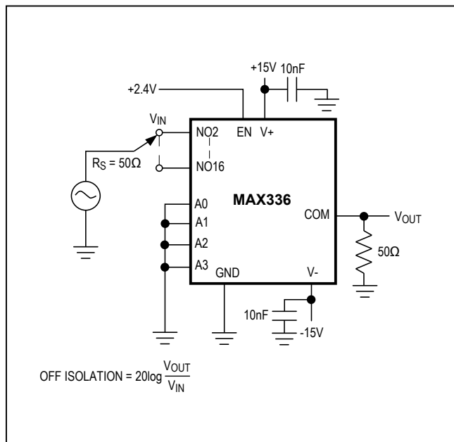
Figure 6. Off Isolation
