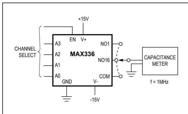
Figure 8. NO/COM Capacitance
