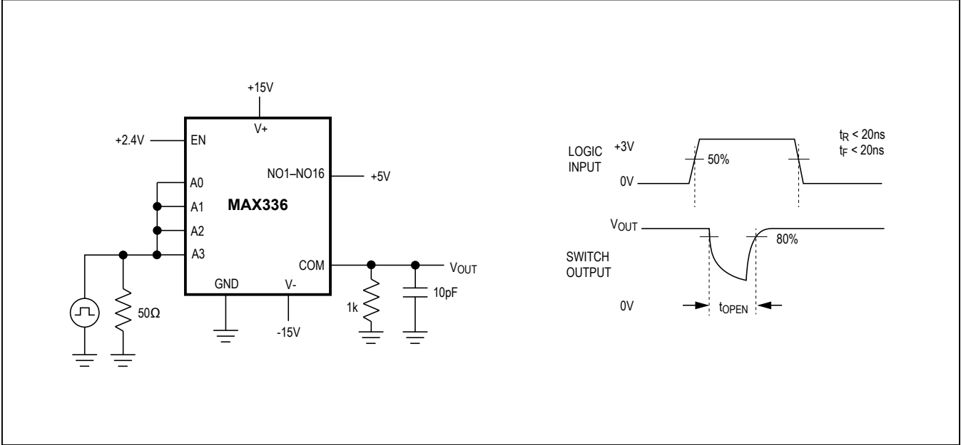
Figure 4. Break-Before-Make Interval
