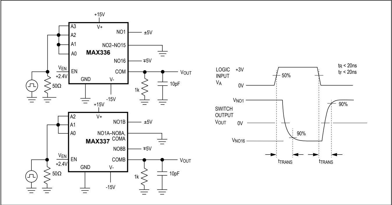
Figure 2. Transition Time
