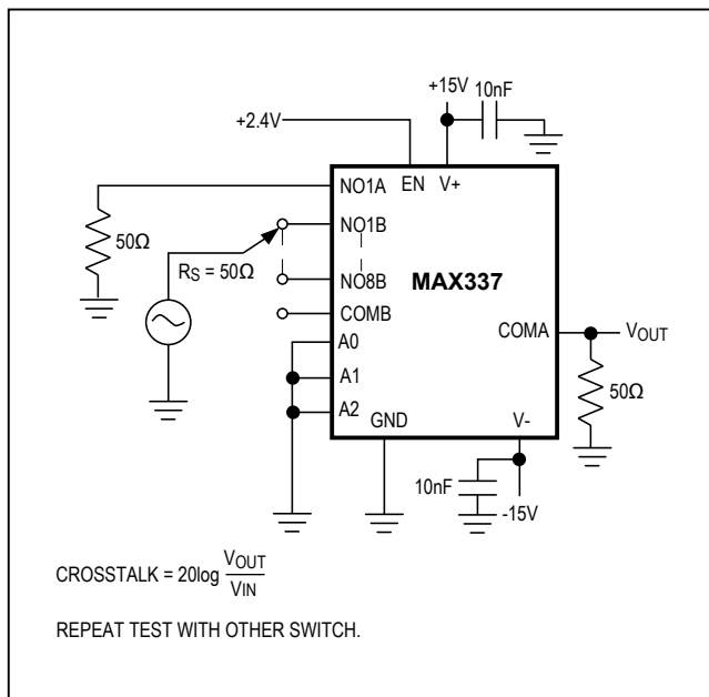
Figure 7. Crosstalk
