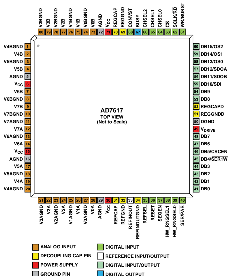
Figure 7. Pin Configuration
