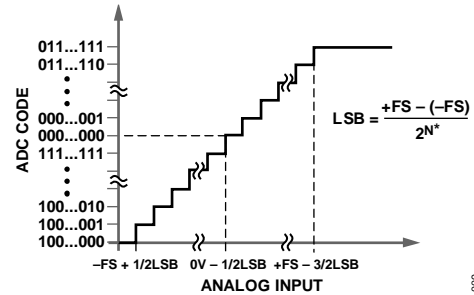
Figure 47. Transfer Characteristics
