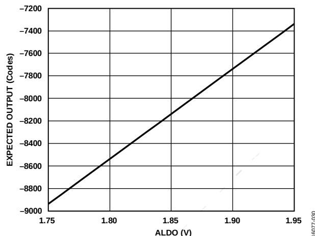
Figure 68. ALDO Diagnostic Transfer Function
