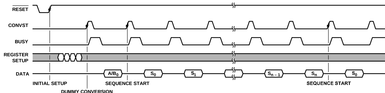
Figure 63. Software Mode Sequencer Configuration
