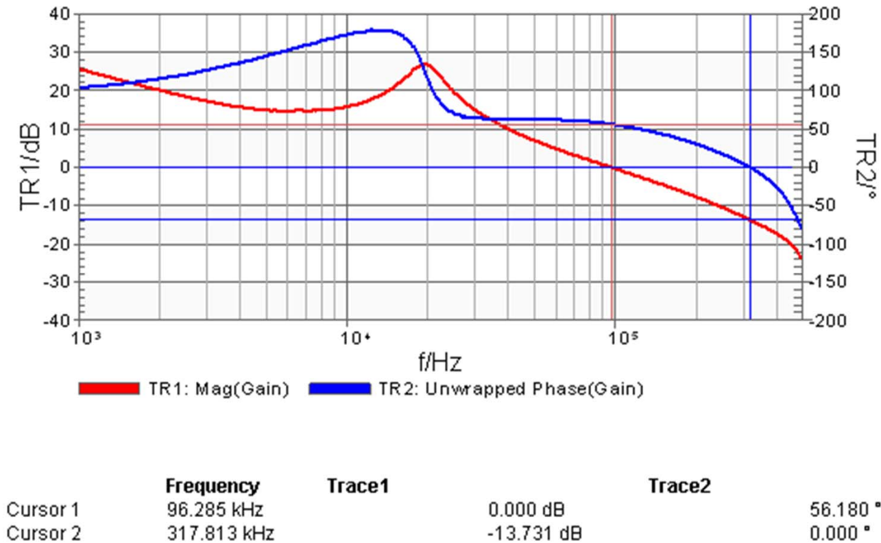
Fig.17: Bode Plot of CH1 at 6A load: Fo = 96.3 kHz; Phase Margin = 56.2°; Gain Margin = 13.7dB
