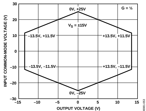
Figure 9. Input Common-Mode Voltage vs. Output Voltage, Gain = \frac{1}{2} , \pm 15\text{ V} Supplies
