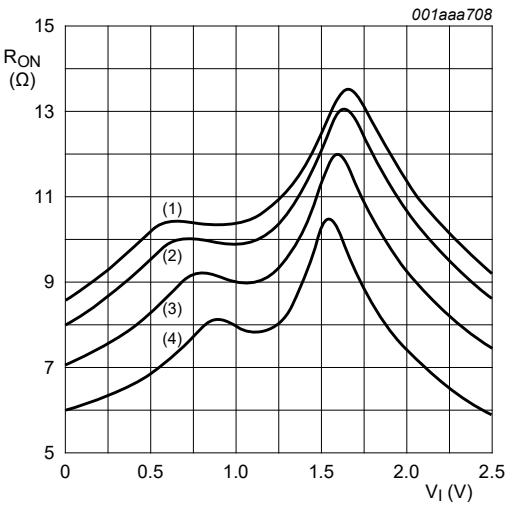
V_{CC} = 2.5\text{ V} 1. T_{amb} = 125\text{ }^{\circ}\text{C} 2. T_{amb} = 85\text{ }^{\circ}\text{C} 3. T_{amb} = 25\text{ }^{\circ}\text{C} 4. T_{amb} = -40\text{ }^{\circ}\text{C}
