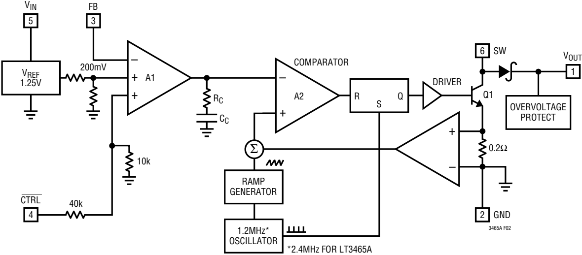
Figure 2. LT3465 Block Diagram
