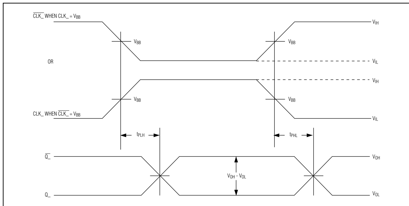
Figure 3. Single-Ended Input ( \text{CLK}_- , \overline{\text{CLK}}_- ) to Output ( \text{Q}_- , \overline{\text{Q}}_- ) Delay Timing Diagram
