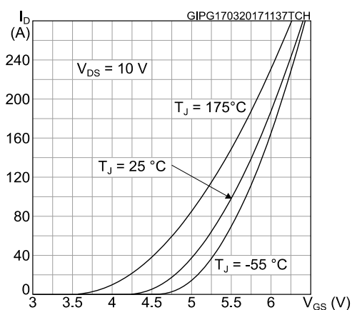
Figure 5: Transfer characteristics
