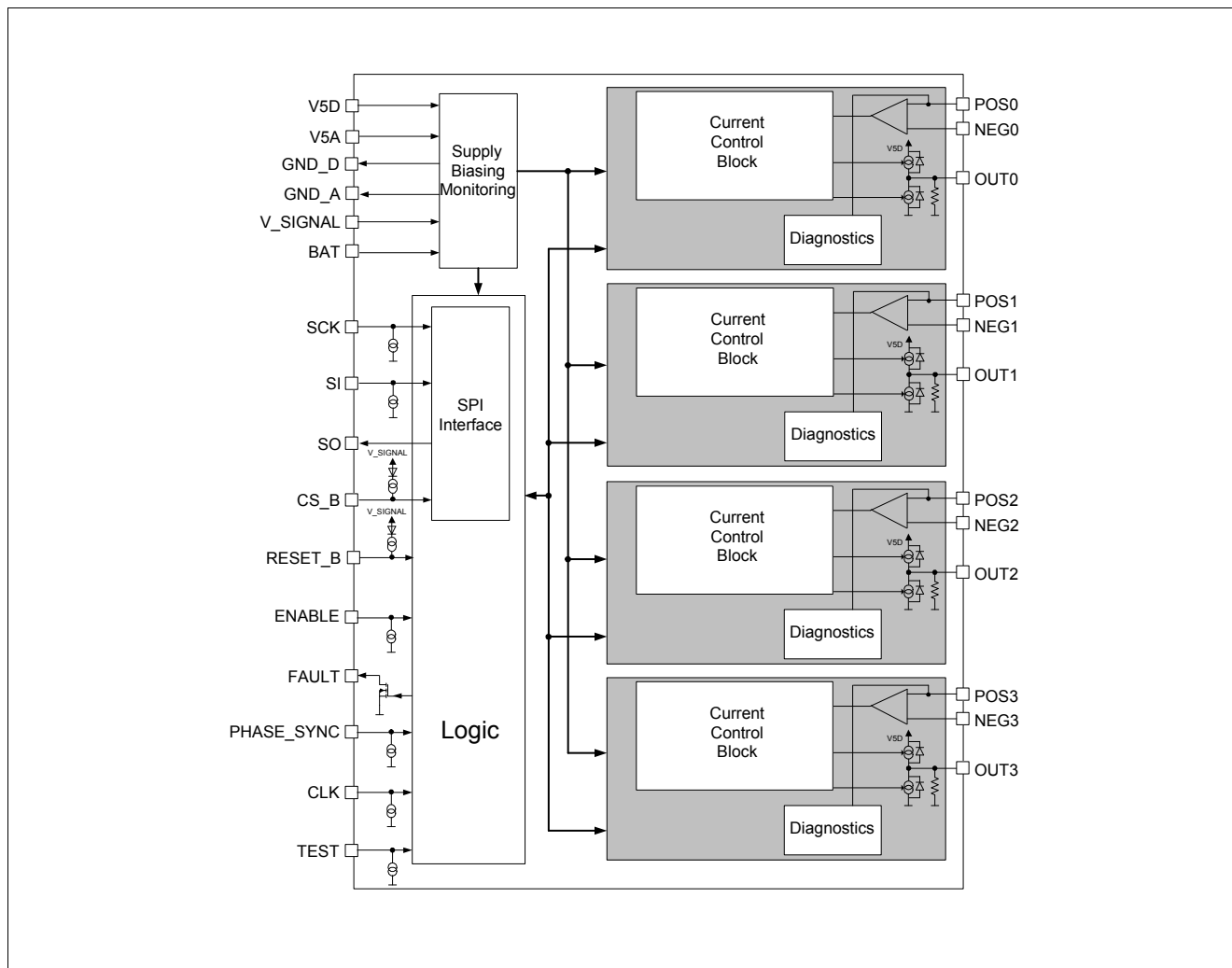
Figure 7 Block Diagram
