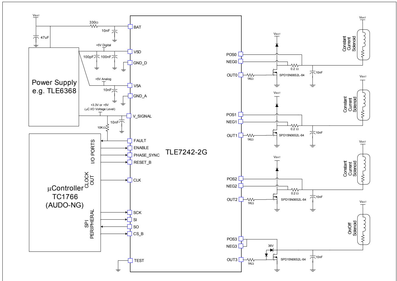
Figure 18 Application Diagram
