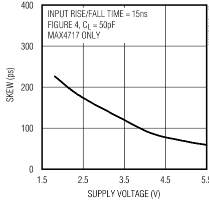
SKEW vs. SUPPLY VOLTAGE
