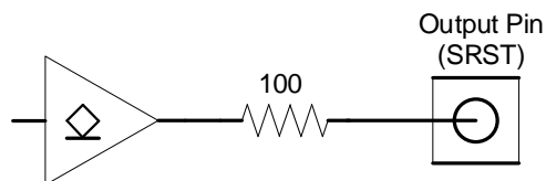
Figure 5. JTAG-HS3 pin 14 output buffer.
