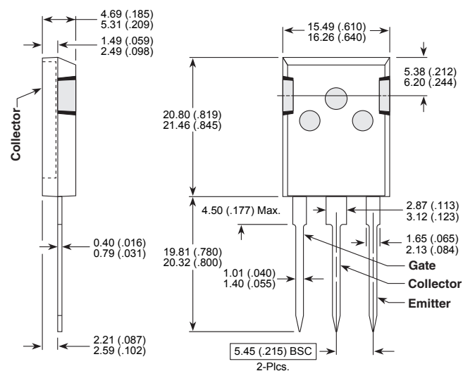
T-MAX™ (B2) Package Outline
