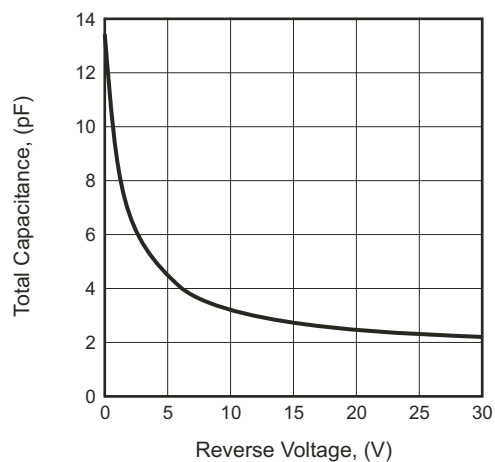
Fig.3 - Total Capacitance
