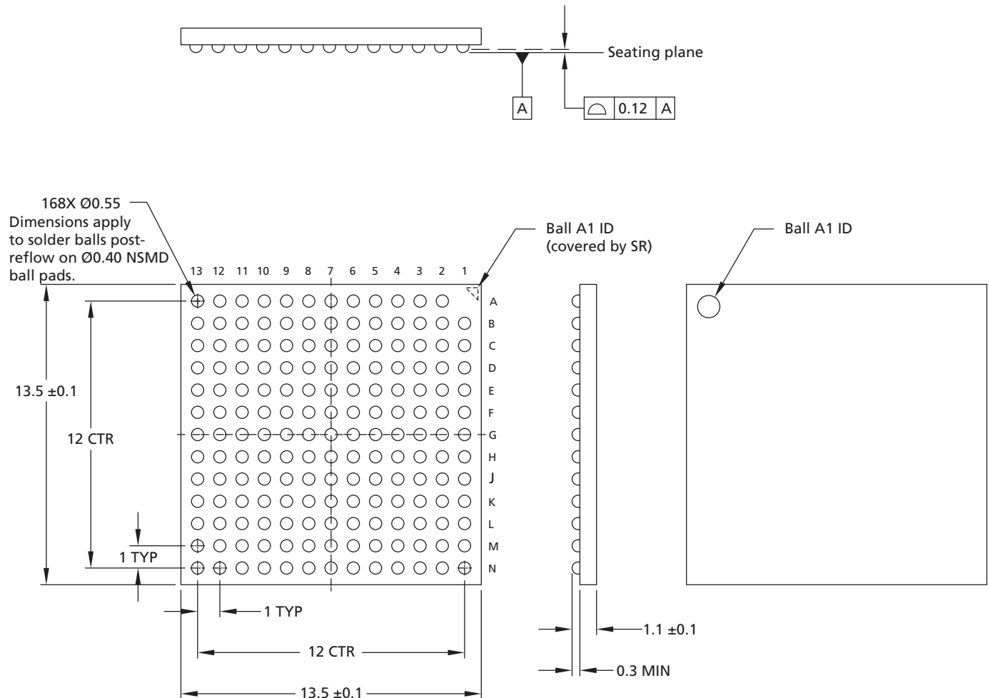
Figure 5: 168-Ball BGA
