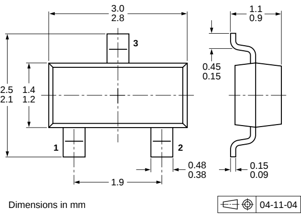
Fig 9. Package outline SOT23 (TO-236AB)
