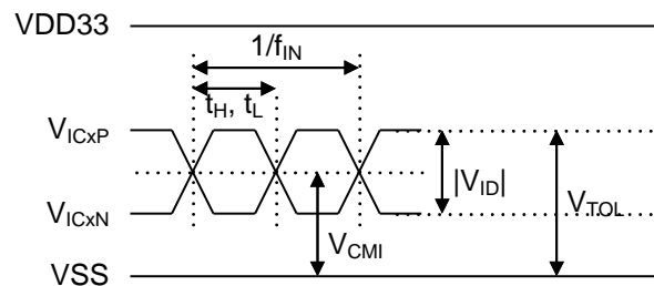
Figure 21 - Electrical Characteristics: Clock Inputs
