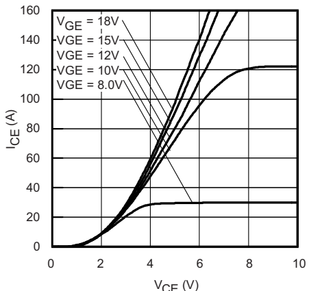
Fig. 6 - Typical IGBT Output Characteristics T_J = 25\text{ °C} ; t_p = 80\text{ }\mu\text{s}
