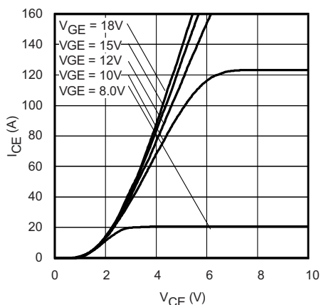
Fig. 5 - Typical IGBT Output Characteristics T_J = -40\text{ °C} ; t_p = 80\text{ }\mu\text{s}
