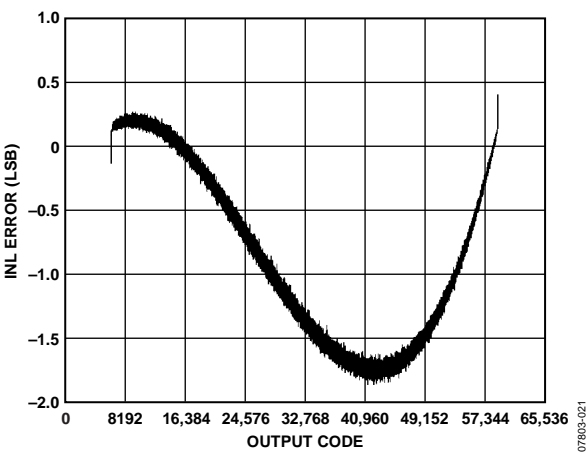
Figure 21. INL with f_{IN} = 2.4\text{ MHz}
