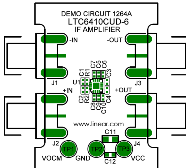
Figure 1. DC1264 Four-Port Evaluation Board
