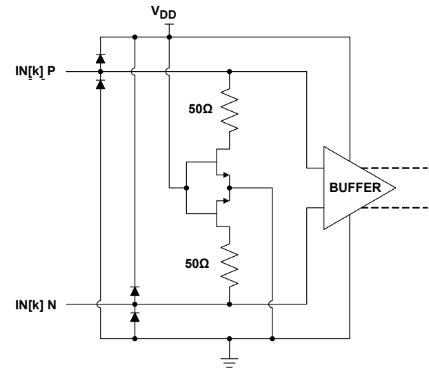
FIGURE 25. CML INPUT EQUIVALENT CIRCUIT FOR THE QLx4600-SL30
