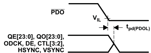
Figure 8. Delay From PDO Low to Hi-Z Outputs
