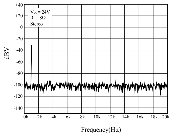
Figure 21 Spectrum at -60dB Signal Input Level
