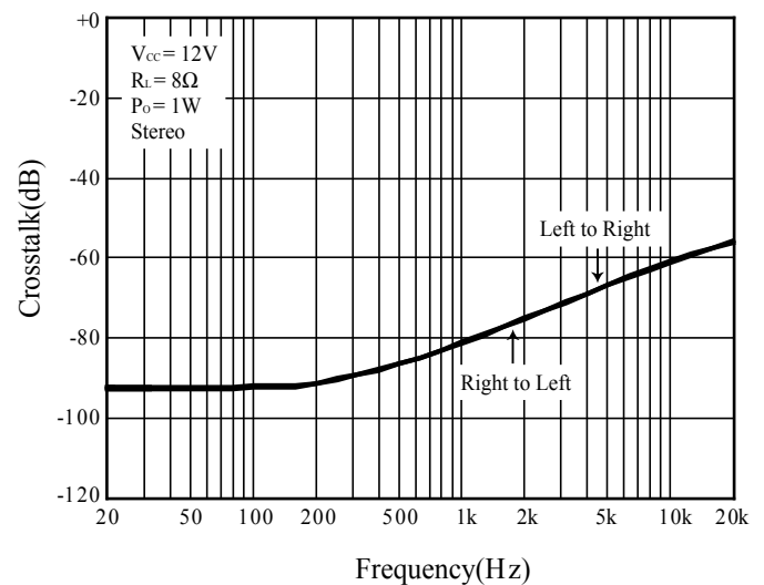
Figure 19 Cross-Talk
