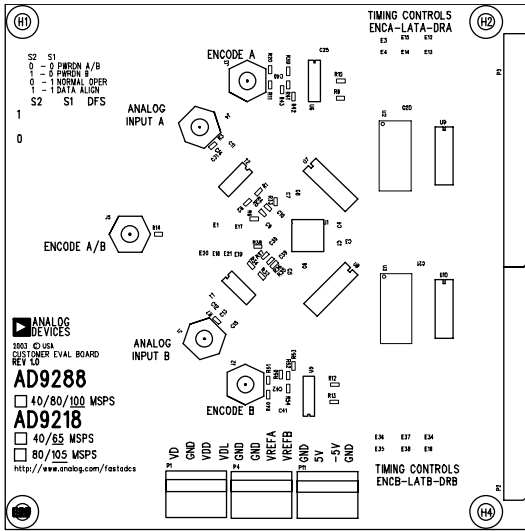
Figure 47. Top Silkscreen
