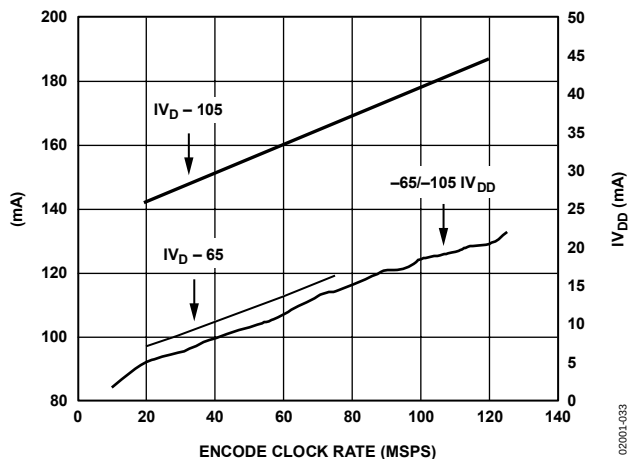
Figure 33. I_{VD} and I_{VD} vs. Encode Rate ( A_{IN} = 10.3 MHz, @ -0.5 dBFS), -65 MSPS/ -105 MSPS Grade C_I = 5 pF
