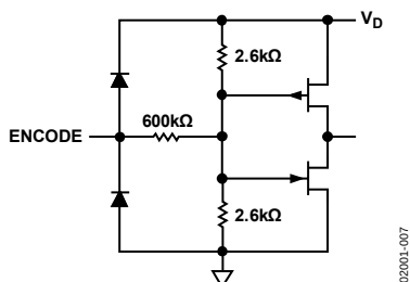
Figure 7. Encode Inputs
