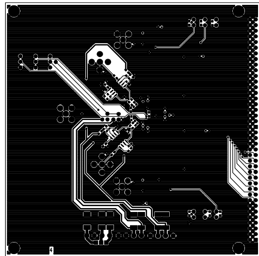
Figure 51. Bottom Routing
