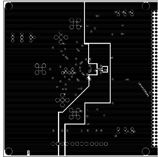
Figure 50. Split Power Plane
