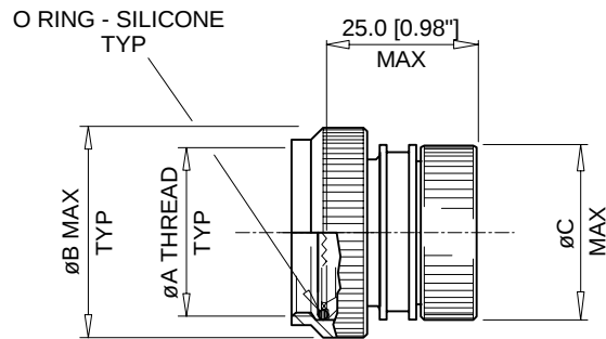
STRAIGHT ADAPTOR
