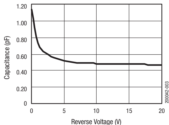
Figure 3. SMS3923 Series Total Capacitance vs Reverse Voltage
