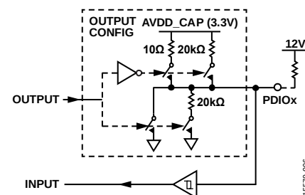
Figure 10. Programmable Driver Input/Output
