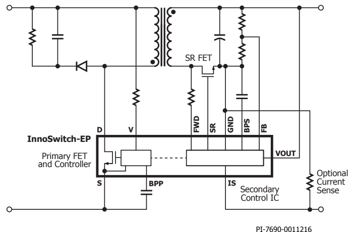
Figure 1. Typical Application/Performance.
