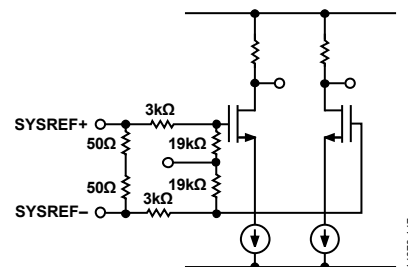
Figure 153. SYSREF \pm Input Circuit for the 11 mm \times 11 mm 169-Ball BGA
