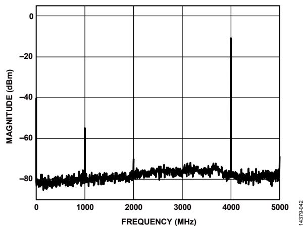
Figure 98. Single-Tone Spectrum at f_{OUT} = 4000 MHz (FIR85 Enabled)
