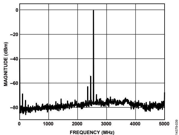
Figure 95. Single-Tone Spectrum at f_{OUT} = 2350 MHz (FIR85 Enabled)
