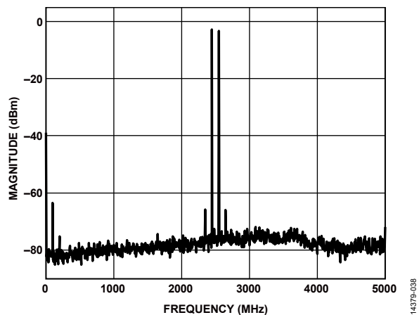
Figure 94. Single-Tone Spectrum at f_{OUT} = 2350 MHz
