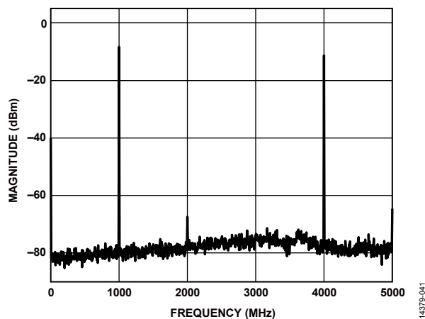
Figure 97. Single-Tone Spectrum at f_{OUT} = 4000 MHz
