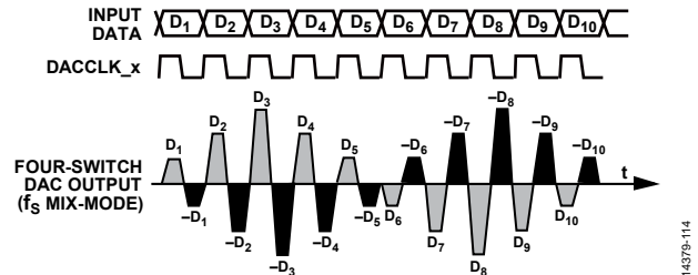
Figure 182. Mix-Mode Waveform
