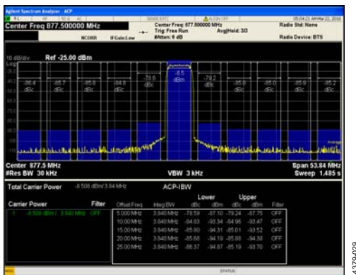
Figure 84. Single-Carrier W-CDMA at 877.5 MHz
