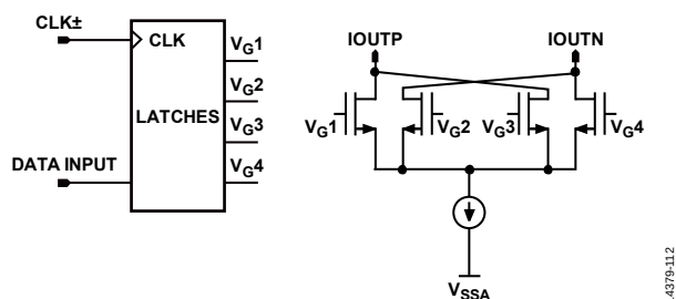
Figure 180. Quad-Switch Architecture
