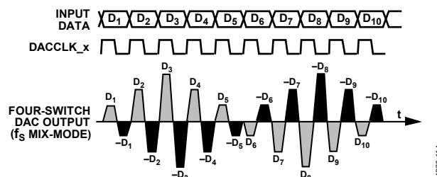
Figure 182. Mix-Mode Waveform
