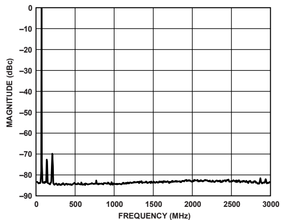
Figure 39. Single Carrier at 70 MHz Output
