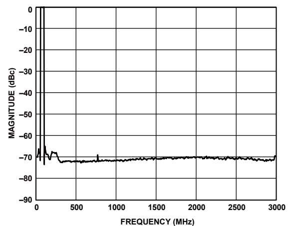
Figure 41. Eight Carriers at 70 MHz Output
