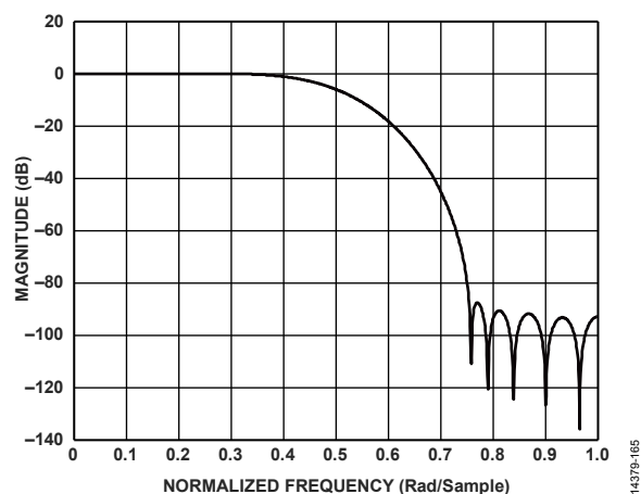
Figure 171. FIR85 2x Half-Band 45% Filter Response
