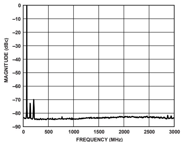
Figure 40. Four Carriers at 70 MHz Output
