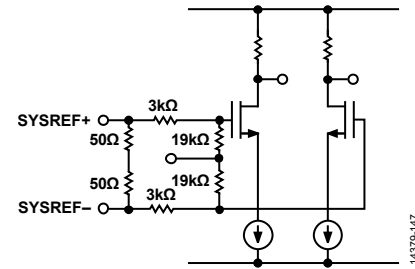
Figure 153. SYSREF \pm Input Circuit for the 11 mm \times 11 mm 169-Ball BGA
