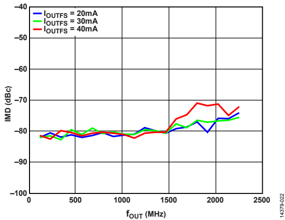
Figure 75. IMD vs. f_{OUT} over DAC I_{OUTFS}
