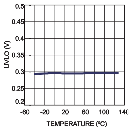
UVLO vs. Temperature
