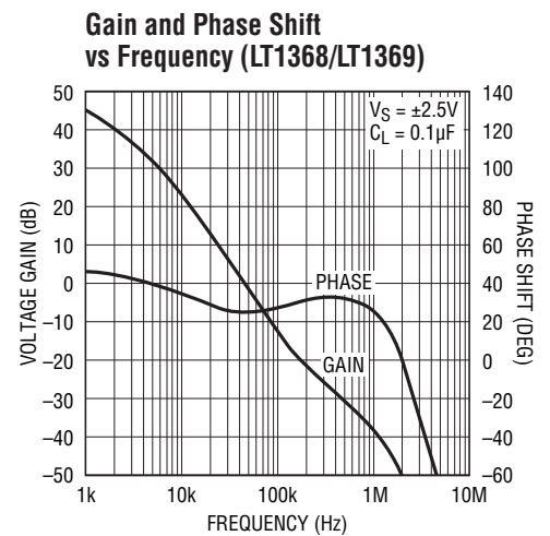
LT1366 TPC15
