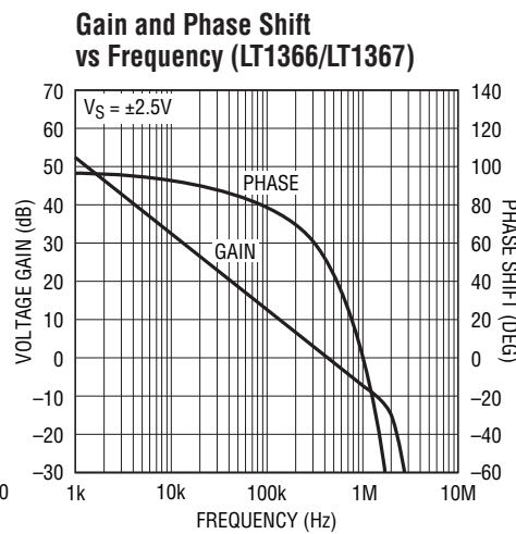
LT1366 TPC14
