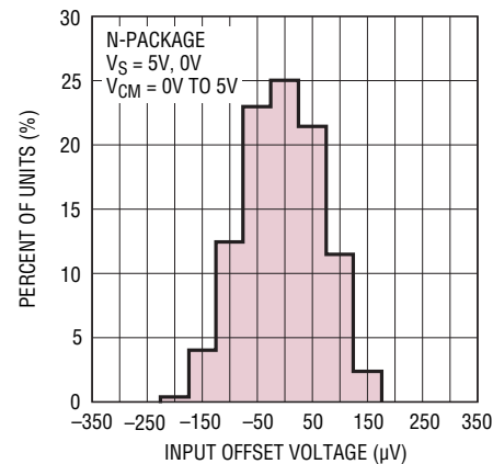
\Delta V_{OS} -Shift Between PNP and NPN Stages (LT1366/LT1368)
