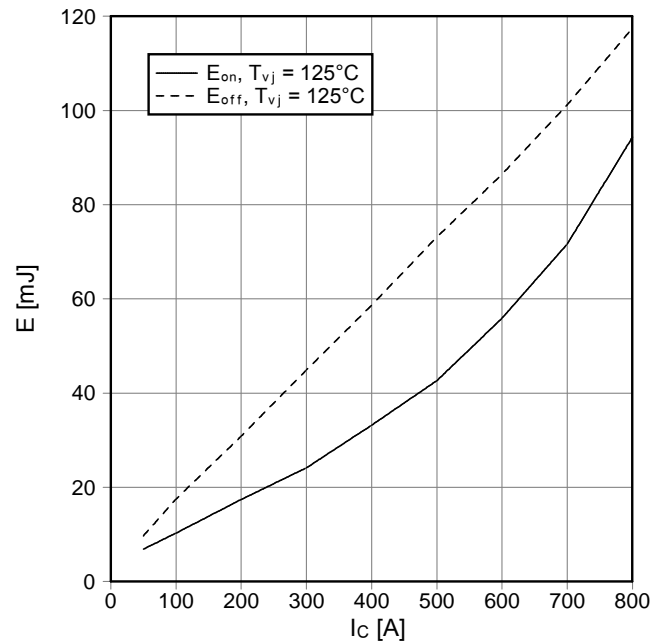
Schaltverluste IGBT-Wechselr. (typisch) switching losses IGBT-inverter (typical) E_{on} = f(I_c), E_{off} = f(I_c) V_{GE} = \pm 15\text{ V}, R_{Gon} = 1,8\ \Omega, R_{Goff} = 1,8\ \Omega, V_{CE} = 600\text{ V}
