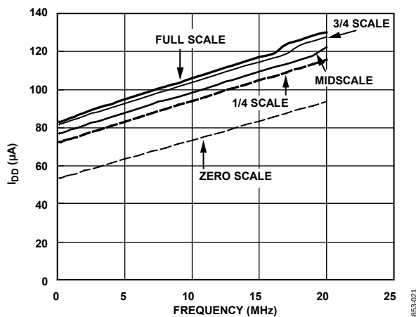
Figure 22. I_{DD} vs. SCLK vs. Code
