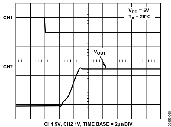
Figure 21. Exiting Power-Down Mode
