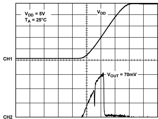
CH1 1V, CH2 20mV, TIME BASE = 20µs/DIV
