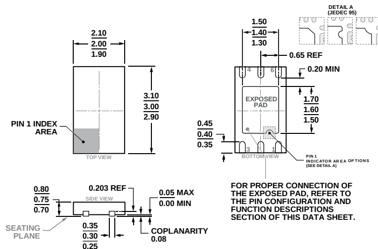
Figure 55. 6-Lead Lead Frame Chip Scale Package [LFCSP] 2.00 x 3.00 mm Body and 0.75 mm Package Height (CP-6-5)
